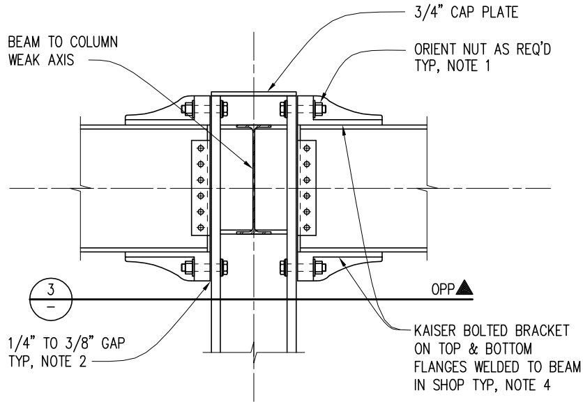
TYPICAL ROOF BRACKET CONNECTION (N 3.1 BRACKET SHOWN)
