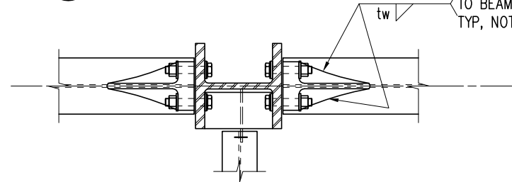
BRACKET CONNECTION PLAN
