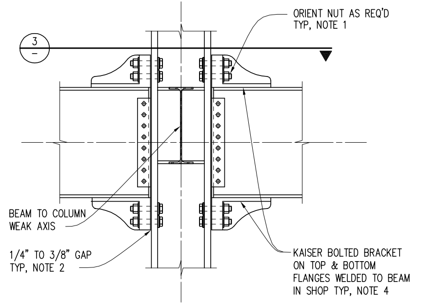
TYPICAL FLOOR BRACKET CONNECTION (N 2.1 BRACKET SHOWN)
